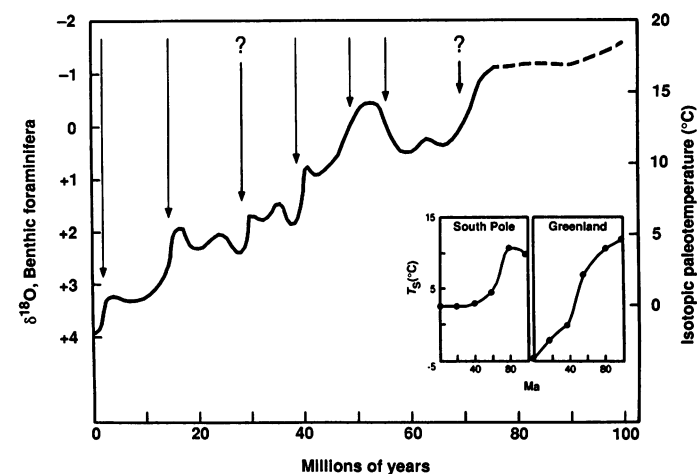
Fig. 5. Climate steps during the last 100 Ma in the oxygen isotope record, along with climate model simulations (inset) suggesting that the long-term trend in climate in key areas is strongly influenced by plate tectonic-induced changes ( T_s = summer temperature). Oxygen isotope record from (92), modified by information from (37, 48, 81); climate simulations from (20).
