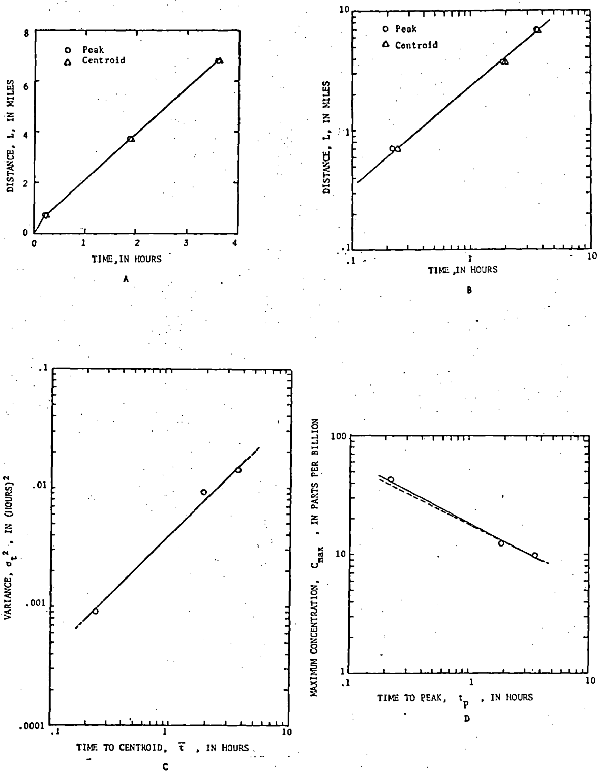
Figure 24.-Dispersion data for case 17, Bear Creek. A. Travel time of the peak and centroid of the tracer cloud, cartesian coordinates. B. Travel time of the peak and centroid of the tracer, logarithmic coordinates. C. Time variance of the tracer concentration distribution plotted against time to centroid. D. Maximum concentration plotted against time to peak. The dashed line indicates the slope for the relation for a Fickian process.
