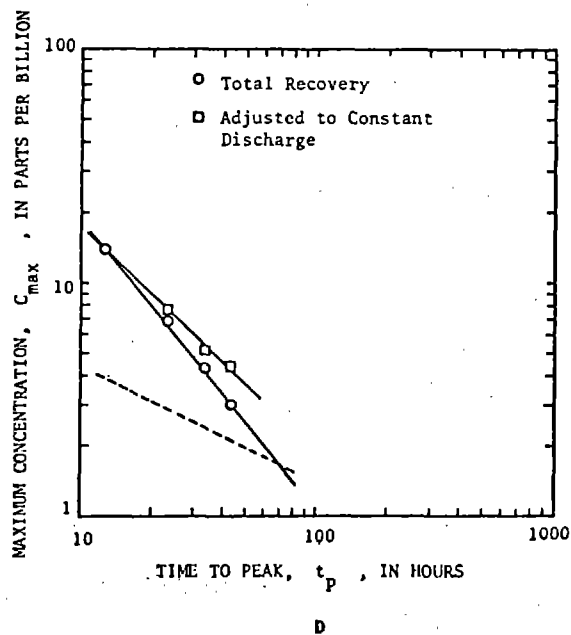
Figure 12.-Dispersion data for case 5, Monocacy River. A. Travel time of the peak and centroid of the tracer cloud, cartesian coordinates. B. Travel time of the peak and centroid of the tracer, logarithmic coordinates. C. Time variance of the tracer concentration distribution plotted against time to centroid. D. Maximum concentration plotted against time to peak. The dashed line indicates the slope for the relation for a Fickian process.
