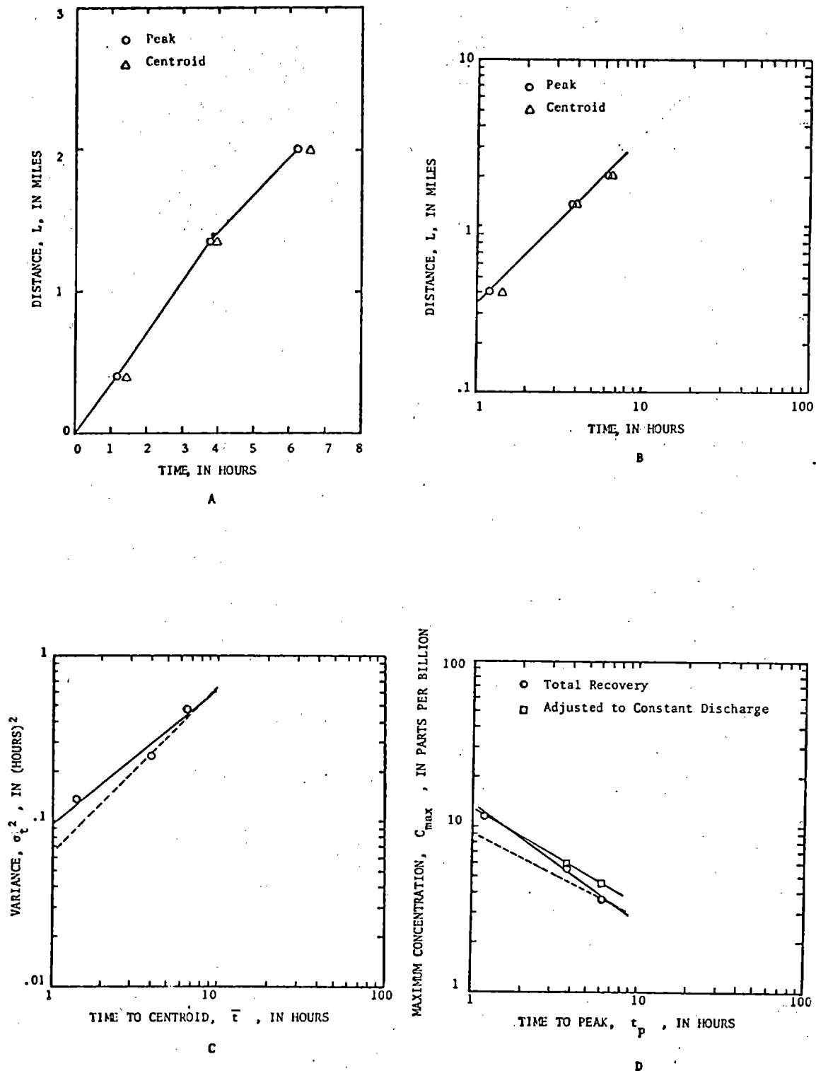
Figure 23.-Dispersion data for case 16, Difficult Run. A. Travel time of the peak and centroid of the tracer cloud, cartesian coordinates. B. Travel time of the peak and centroid of the tracer, logarithmic coordinates. C. Time variance of the tracer concentration distribution plotted against time to centroid. D. Maximum concentration plotted against time to peak. The dashed line indicates the slope for the relation for a Fickian process.
