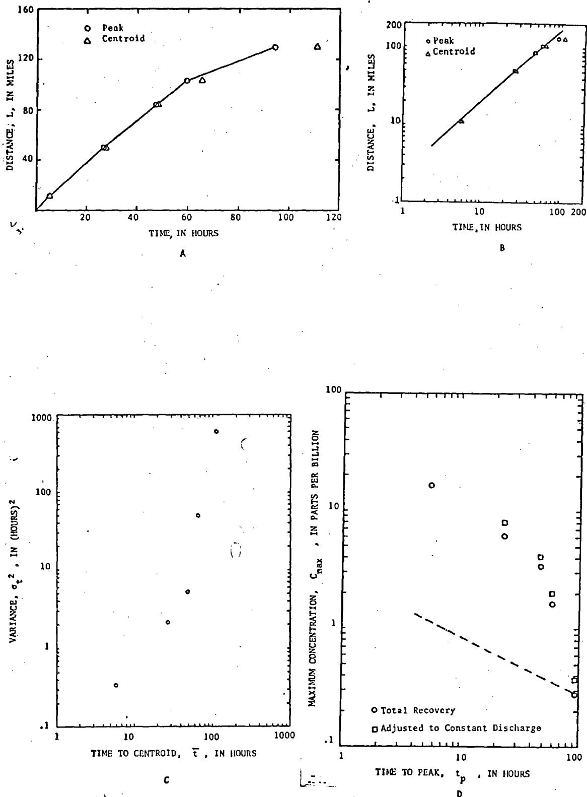
Figure 38.-Dispersion data for case 31, Sabine River. A. Travel time of the peak and centroid of the tracer cloud, cartesian coordinates. B. Travel time of the peak and centroid of the tracer, logarithmic coordinates. C. Time variance of the tracer concentration distribution plotted against time to centroid. D. Maximum concentration plotted against time to peak. The dashed line indicates the slope for the relation for a Fickian process.
