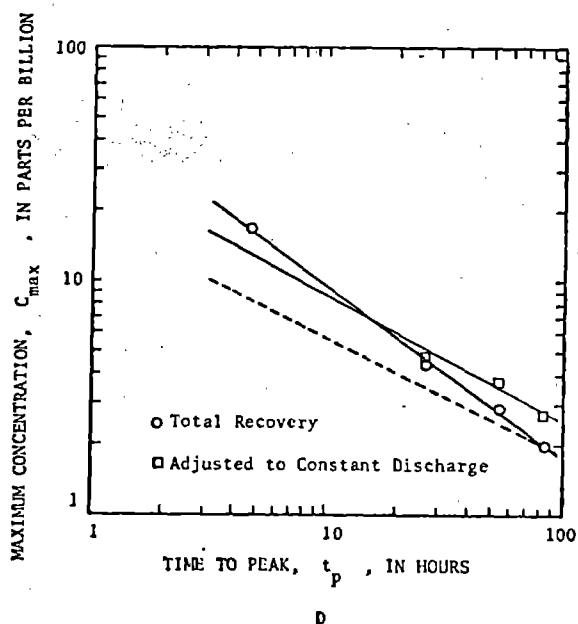
Figure 35.-Dispersion data for case 28, Red River. A. Travel time of the peak and centroid of the tracer cloud, cartesian coordinates. B. Travel time of the peak and centroid of the tracer, logarithmic coordinates. C. Time variance of the tracer concentration distribution plotted against time to centroid. D. Maximum concentration plotted against time to peak. The dashed line indicates the slope for the relation for a Fickian process.
