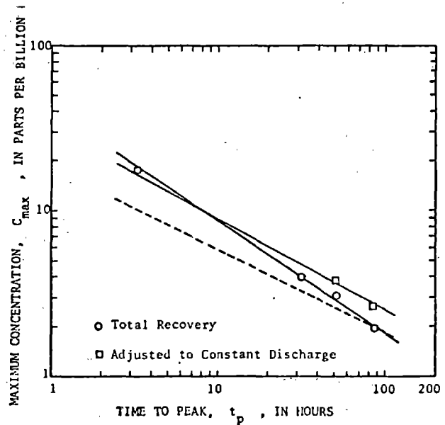
Figure 34.—Dispersion data for case 27, Red River. A. Travel time of the peak and centroid of the tracer cloud, cartesian coordinates. B. Travel time of the peak and centroid of the tracer, logarithmic coordinates. C. Time variance of the tracer concentration distribution plotted against time to centroid. D. Maximum concentration plotted against time to peak. The dashed line indicates the slope for the relation for a Fickian process.
