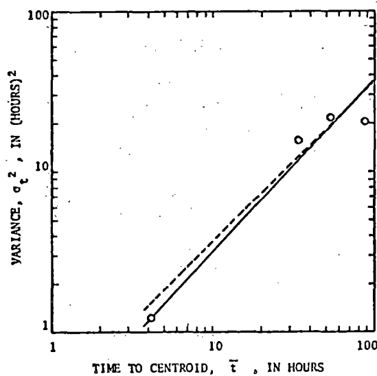
Figure 34.—Dispersion data for case 27, Red River. A. Travel time of the peak and centroid of the tracer cloud, cartesian coordinates. B. Travel time of the peak and centroid of the tracer, logarithmic coordinates. C. Time variance of the tracer concentration distribution plotted against time to centroid. D. Maximum concentration plotted against time to peak. The dashed line indicates the slope for the relation for a Fickian process.
