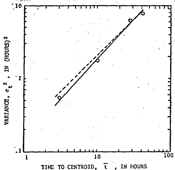
Figure 10.-Dispersion data for case 3, Antietam Creek. A. Travel time of the peak and centroid of the tracer cloud, cartesian coordinates. B. Travel time of the peak and centroid of the tracer, logarithmic coordinates. C. Time variance of the tracer concentration distribution plotted against time to centroid. D. Maximum concentration plotted against time to peak. The dashed line indicates the slope for the relation for a Fickian process.
