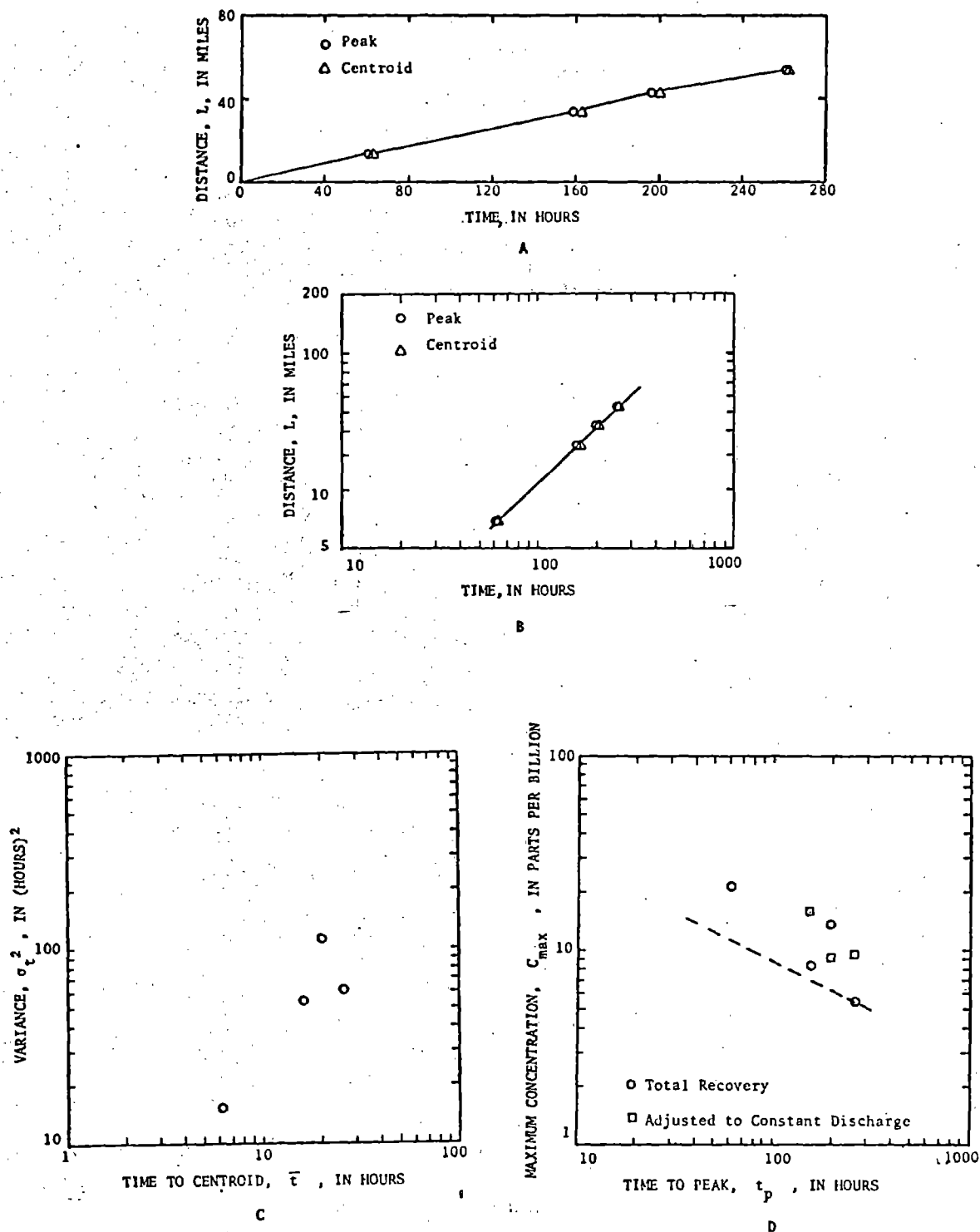
Figure 39.-Dispersion data for case 32, Sabine River. A. Travel time of the peak and centroid of the tracer cloud, cartesian coordinates. B. Travel time of the peak and centroid of the tracer, logarithmic coordinates. C. Time variance of the tracer concentration distribution plotted against time to centroid. D. Maximum concentration plotted against time to peak. The dashed line indicates the slope for the relation for a Fickian process.
