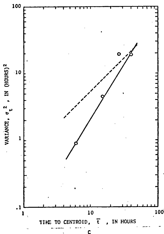
Figure 18.-Dispersion data for case 11, Conococheague Creek. A. Travel time of the peak and centroid of the tracer cloud, cartesian coordinates. B. Travel time of the peak and centroid of the tracer, logarithmic coordinates. C. Time variance of the tracer concentration distribution plotted against time to centroid. D. Maximum concentration plotted against time to peak. The dashed line indicates the slope for the relation for a Fickian process.
