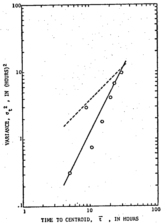
Figure 20.-Dispersion data for case 13, Chattahoochee River. A. Travel time of the peak and centroid of the tracer cloud, cartesian coordinates. B. Travel time of the peak and centroid of the tracer, logarithmic coordinates. C. Time variance of the tracer concentration distribution plotted against time to centroid. D. Maximum concentration plotted against time to peak. The dashed line indicates the slope for the relation for a Fickian process.
