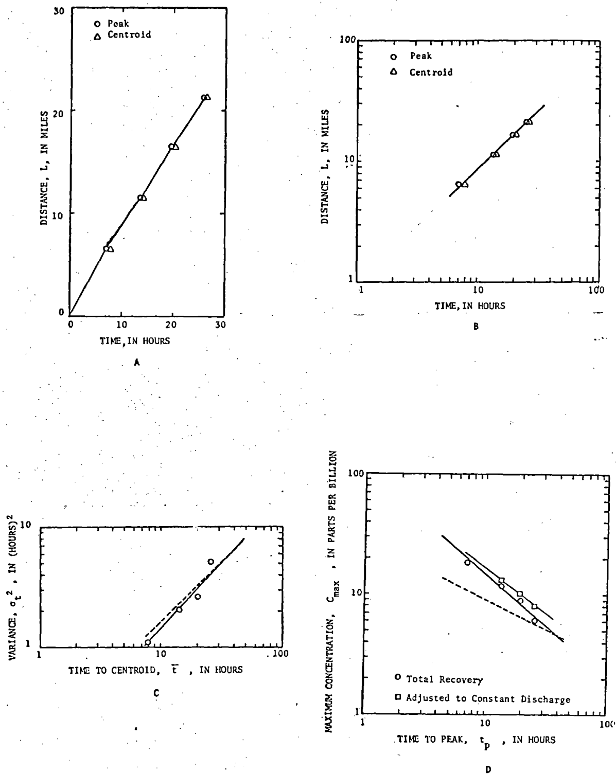
Figure 14.-Dispersion data for case 7, Monocacy River. A. Travel time of the peak and centroid of the tracer cloud, cartesian coordinates. B. Travel time of the peak and centroid of the tracer, logarithmic coordinates. C. Time variance of the tracer concentration distribution plotted against time to centroid. D. Maximum concentration plotted against time to peak. The dashed line indicates the slope for the relation for a Fickian process.
