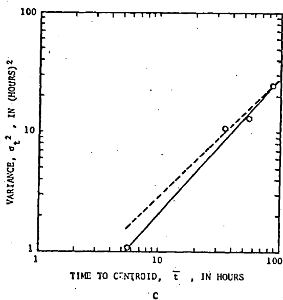
Figure 35.-Dispersion data for case 28, Red River. A. Travel time of the peak and centroid of the tracer cloud, cartesian coordinates. B. Travel time of the peak and centroid of the tracer, logarithmic coordinates. C. Time variance of the tracer concentration distribution plotted against time to centroid. D. Maximum concentration plotted against time to peak. The dashed line indicates the slope for the relation for a Fickian process.
