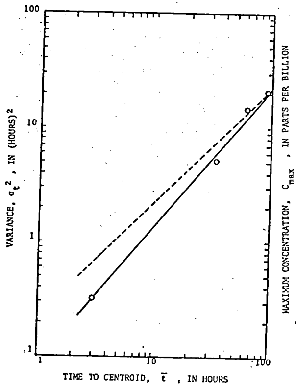
Figure 33.-Dispersion data for case 26, Red River. A. Travel time of the peak and centroid of the tracer cloud, cartesian coordinates. B. Travel time of the peak and centroid of the tracer, logarithmic coordinates. C. Time variance of the tracer concentration distribution plotted against time to centroid. D. Maximum concentration plotted against time to peak. The dashed line indicates the slope for the relation for a Fickian process.
