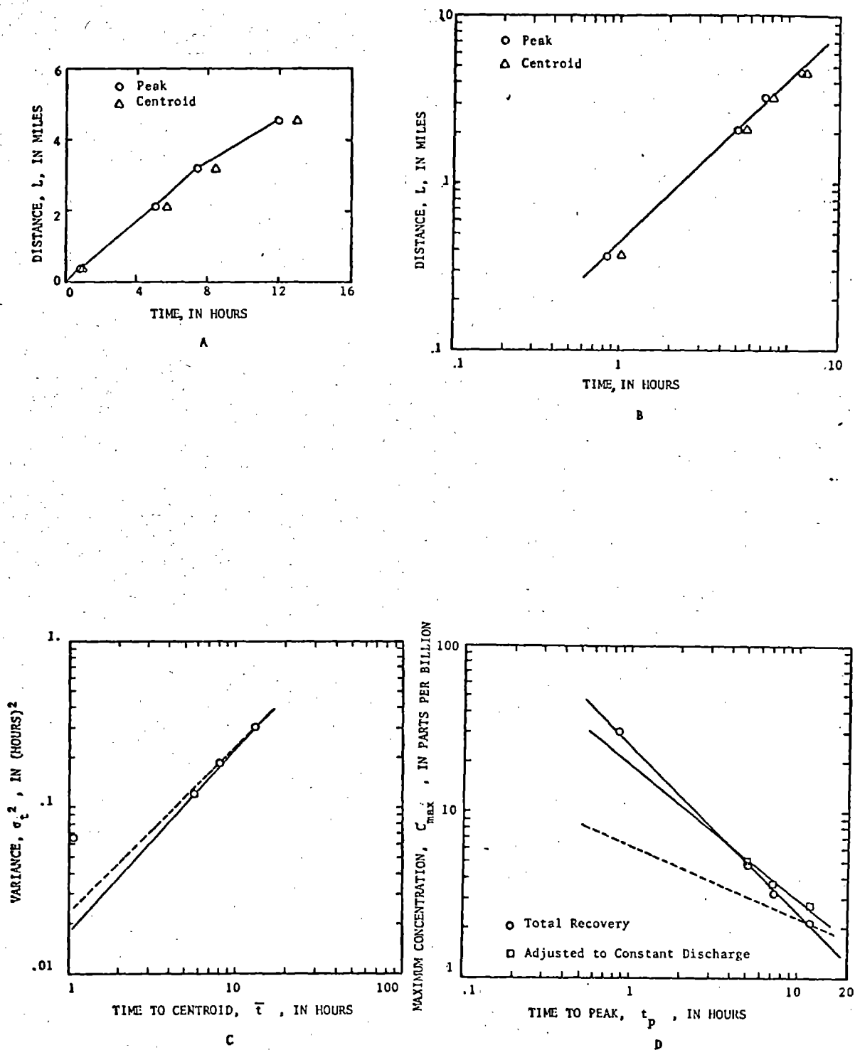
Figure 25.-Dispersion data for case 18, Little Piney Creek. A. Travel time of the peak and centroid of the tracer cloud, cartesian coordinates. B. Travel time of the peak and centroid of the tracer, logarithmic coordinates. C. Time variance of the tracer concentration distribution plotted against time to centroid. D. Maximum concentration plotted against time to peak. The dashed line indicates the slope for the relation for a Fickian process.
