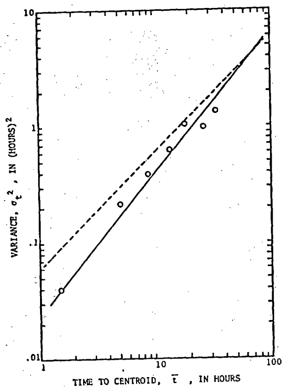
Figure 46.-Dispersion data for case 39, Wind/Bighorn River. A. Travel time of the peak and centroid of the tracer cloud, cartesian coordinates. B. Travel time of the peak and centroid of the tracer, logarithmic coordinates. C. Time variance of the tracer concentration distribution plotted against time to centroid. D. Maximum concentration plotted against time to peak. The dashed line indicates the slope for the relation for a Fickian process.
