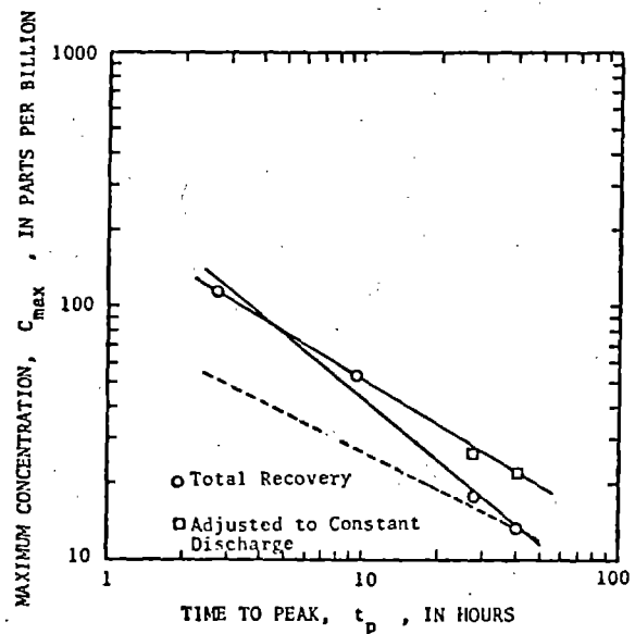
Figure 10.-Dispersion data for case 3, Antietam Creek. A. Travel time of the peak and centroid of the tracer cloud, cartesian coordinates. B. Travel time of the peak and centroid of the tracer, logarithmic coordinates. C. Time variance of the tracer concentration distribution plotted against time to centroid. D. Maximum concentration plotted against time to peak. The dashed line indicates the slope for the relation for a Fickian process.
