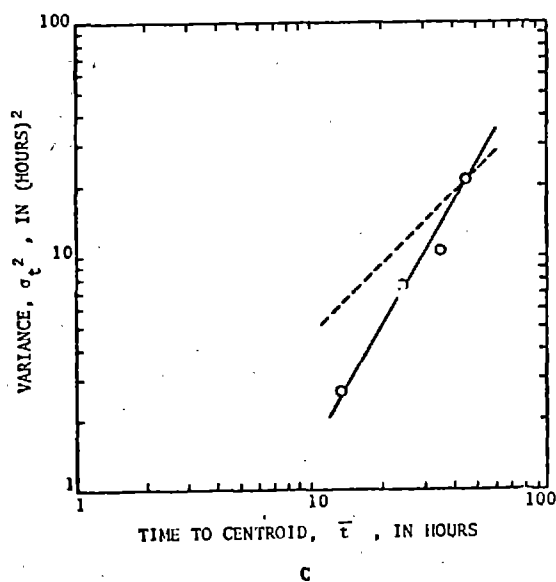
Figure 12.-Dispersion data for case 5, Monocacy River. A. Travel time of the peak and centroid of the tracer cloud, cartesian coordinates. B. Travel time of the peak and centroid of the tracer, logarithmic coordinates. C. Time variance of the tracer concentration distribution plotted against time to centroid. D. Maximum concentration plotted against time to peak. The dashed line indicates the slope for the relation for a Fickian process.
