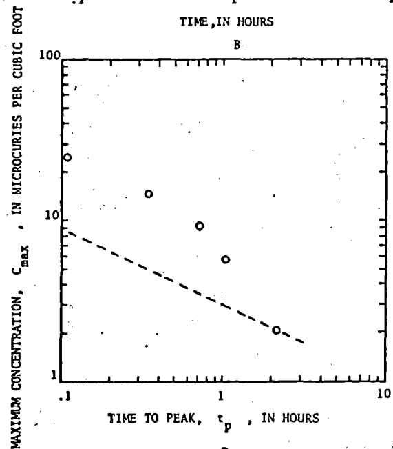
Figure 54.-Dispersion data for case 47, Coachella Canal. A. Travel time of the peak and centroid of the tracer cloud, cartesian coordinates. B. Travel time of the peak and centroid of the tracer, logarithmic coordinates. C. Time variance of the tracer concentration distribution plotted against time to centroid. D. Maximum concentration plotted against time to peak. The dashed line indicates the slope for the relation for a Fickian process.
