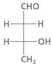
3-Hydroxybutanal
