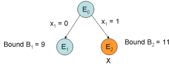
Figure 3: Use of bounds.
