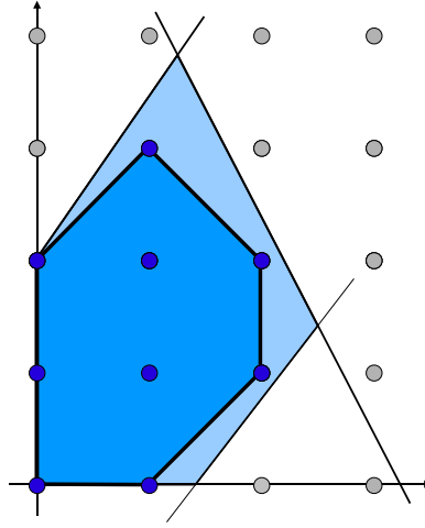
Figure 6: A formulation for a set of integer points and the ideal formulation.
