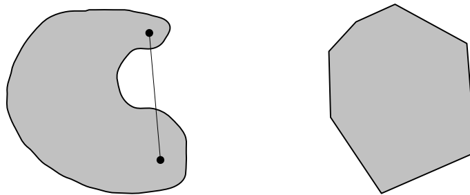
Figure 4: A convex set and a non-convex set.
