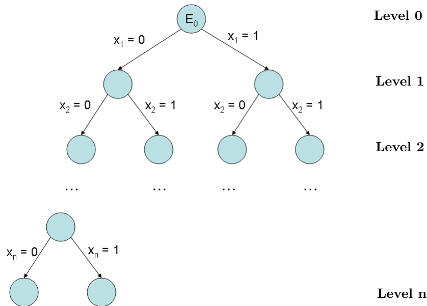
Figure 2: Binary branching.
