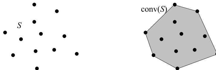
Figure 5: A set and its convex hull.
