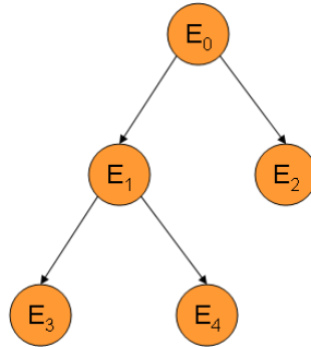
Figure 1: How to generate solutions: the branching operation.
