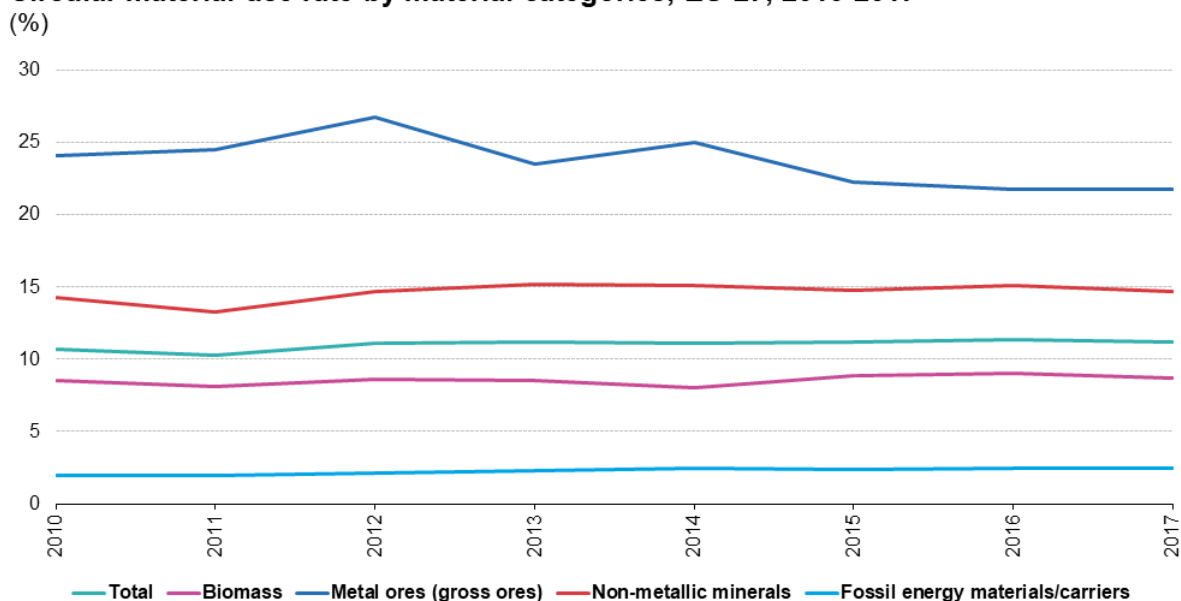
Circular material use rate by material categories, EU-27, 2010-2017
