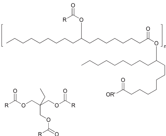
Scheme 2 Two examples of triglyceride derived bio-lubricants. Top: an estolide ester ( R' = \text{H} or 2-ethyl-1-hexyl). Bottom: a partially bio-based synthetic trimethylolpropane ester ( R = \text{fatty acid alkyl} ). 65
