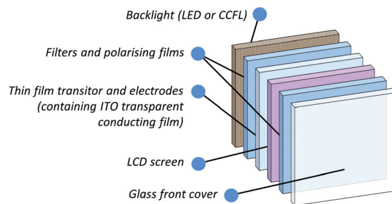
Fig. 8 A simplified, exploded diagram of the layers in a LCD screen. 109,114
