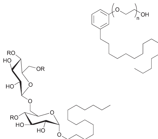
Scheme 4 Top right: a cashew nut shell liquid derived surfactant. 137 Bottom left: an alkyl polyglucoside made from glucose and a fatty alcohol (R = H or glucose). 138
