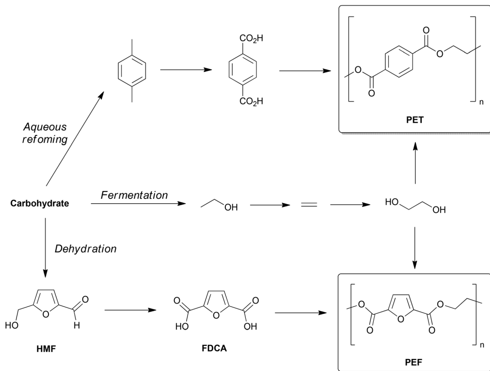
Scheme 5 The synthesis of bio-based polyethylene terephthalate (PET) and polyethylene furanoate (PEF).
