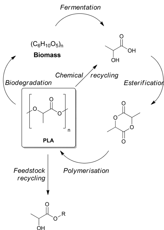
Scheme 6 Chemical recycling options for PLA.
