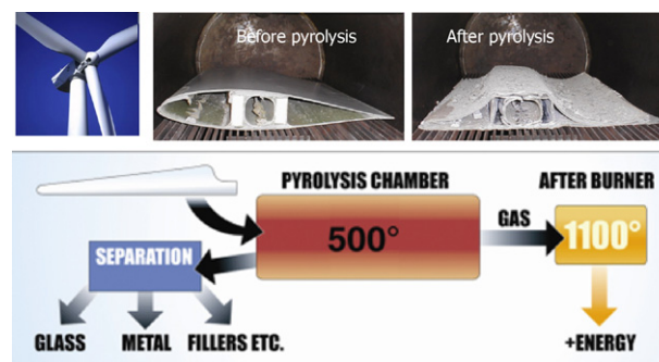
Fig. 6. Illustration of ReFibre process for recycling of wind turbine blades [24].
