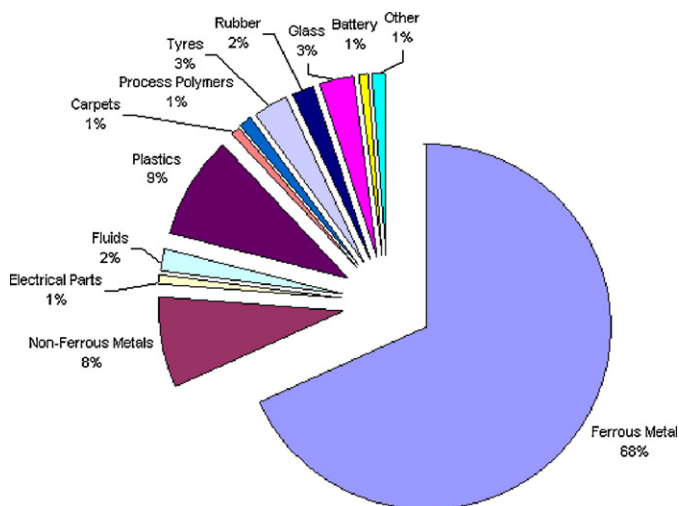
Fig. 8. Average material compositions of a vehicle produced in 2000. http://www.wasteonline.org.uk/resources/InformationSheets/vehicle.htm .
