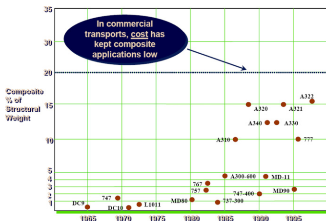
Fig. 7. Composite usage trends in commercial transports and general aviation aircrafts [33].
