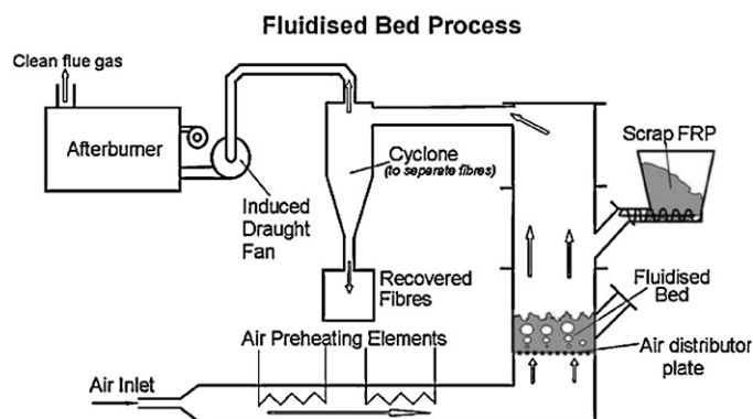
Fig. 5. Fluidised-bed process for fibre and energy recovery (combustion) [12].
