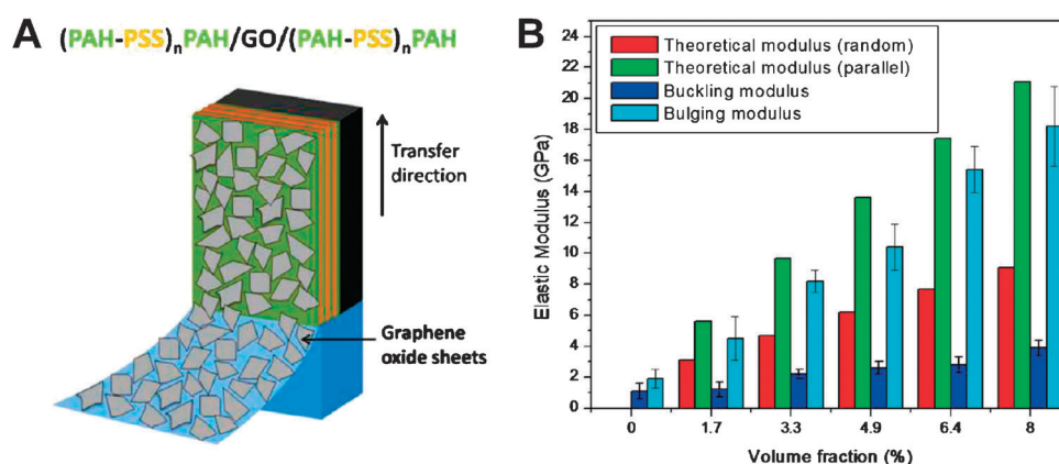
Fig. 4 (A) Schematic illustration of fabrication and assembly of the free-standing GO-LbL film. (B) Plot showing the variation of elastic modulus calculated theoretically (under parallel and random orientation) and that obtained experimentally (using buckling and bulging measurements) with the volume fraction of GO. Reproduced with permission from ref. 215. Copyright 2010, American Chemical Society.
