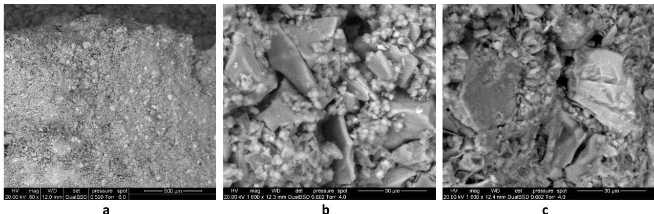
Fig. 4. Microstructural details of V5G5_0.42 sample at increasing magnification.
