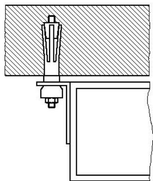
Suspended rectangular duct with expansion plug
