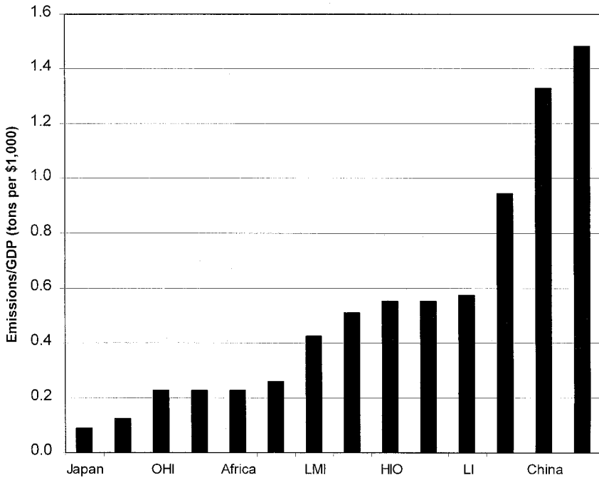
Figure 3.1 Industrial CO 2 -output ratios for thirteen RICE subregions, 1995 For key to regions, see table 3.1.
