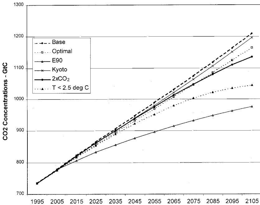
Figure 7.8 CO 2 concentrations: Alternative policies
