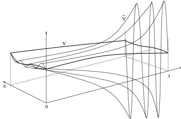
FIGURE 15. An ill-posed Cauchy problem. Here v is a reference solution, while \tilde{v} is a perturbed solution. A small change in the initial data at t = 0 produces a large change in the solution at a later time t > 0 .
