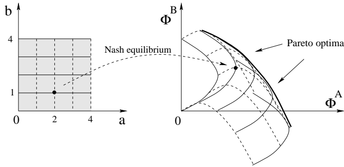
FIGURE 6. The payoff map (a, b) \mapsto (\Phi^A, \Phi^B) for the game (2.7). The Nash equilibrium is (2, 1) , which does not yield a Pareto optimum.
