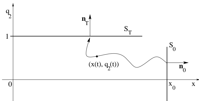
FIGURE 10. The initial and terminal constraints for the optimal control problem (4.41)–(4.43). According to (10.25), at time t = 0 one has (\lambda_1(0), \lambda_2(0)) = \mathbf{n}_0 for some vector \mathbf{n}_0 perpendicular to the manifold S_0 = \{(x, q_2); x = x_0\} . Hence \lambda_2(0) = 0 while \lambda_1(0) can be arbitrary. On the other hand, at time t = T one has (\lambda_1(T), \lambda_2(T)) = \lambda_0(b, 1) + \mathbf{n}_T for some vector \mathbf{n}_T perpendicular to the manifold S_T = \{(x, q_2); q_2 = 1\} . Hence \lambda_1(T) = \lambda_0 b while \lambda_2(T) can be arbitrary.
