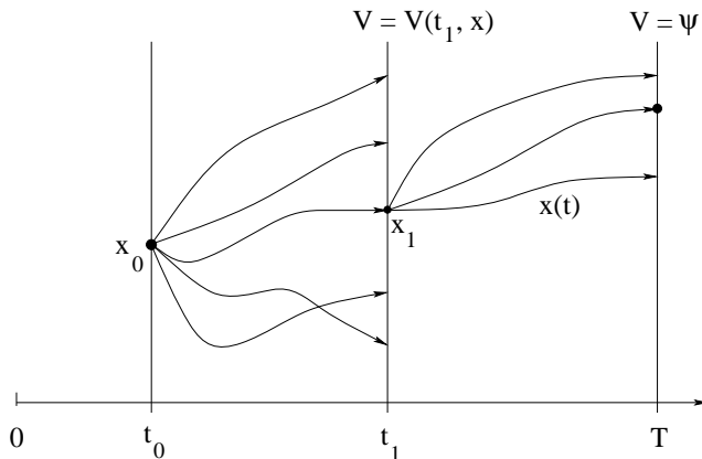
FIGURE 14. An illustration of the dynamic programming principle.
