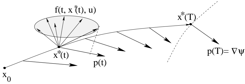
FIGURE 13. An illustration of the Pontryagin maximum principle, in the case where L(t, x, u) \equiv 0 . At each time t \in [0, T] , among all possible velocities \dot{x} = f(t, x^*(t), u) , u \in U (shaded set), the optimal choice is the one that maximizes the inner product with the adjoint vector p(t) .
