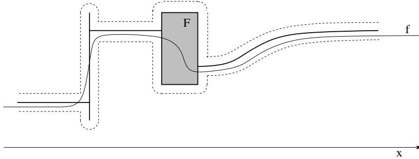
FIGURE 12. An upper semicontinuous multifunction F with convex values, the \varepsilon -neighborhood of its graph, and a continuous \varepsilon -approximate selection f .
