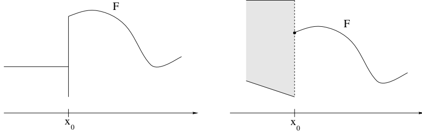
FIGURE 11. Left: the graph of an upper semicontinuous function. Here F(x_0) contains an entire segment, while F(x) is single-valued for x \neq x_0 . Right: the graph of a lower semicontinuous function. Here F(x_0) consists of just one point, while F(x) is multivalued for x < x_0 .
