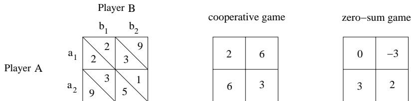
FIGURE 9. Left: the payoffs of a bi-matrix game, where each player has two options. This can be represented as the sum of a cooperative game where both players have exactly the same payoff, plus a zero-sum game. In the center is the matrix of payoffs \Phi^{\sharp} , on the right is the matrix of payoffs \Phi^{\flat} .
