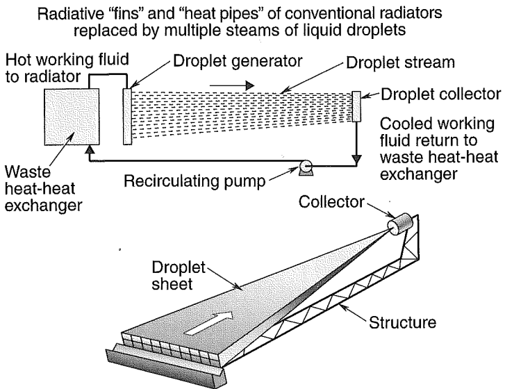
Fig. 6.15. Liquid-droplet radiator.
