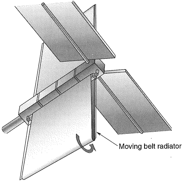
Fig. 6.14. Moving-belt radiator.
